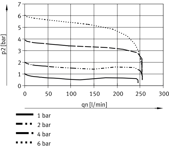
Standard flow rate q_n as a function of output pressure p_2 ( p_1 = 7 \text{ bar} ) – MS2-LFR-QS6-...-B (grade of filtration: 5 \mu\text{m} )
