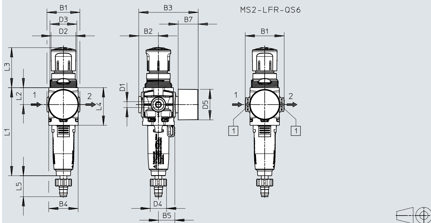
Dimensions – MS2-LFR-...-B with pressure gauge
