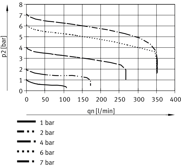
Standard flow rate q_n as a function of output pressure p_2 ( p_1 = 10 \text{ bar} ) – MS2-LFR- M5-...-B (grade of filtration: 5 \mu\text{m} )
